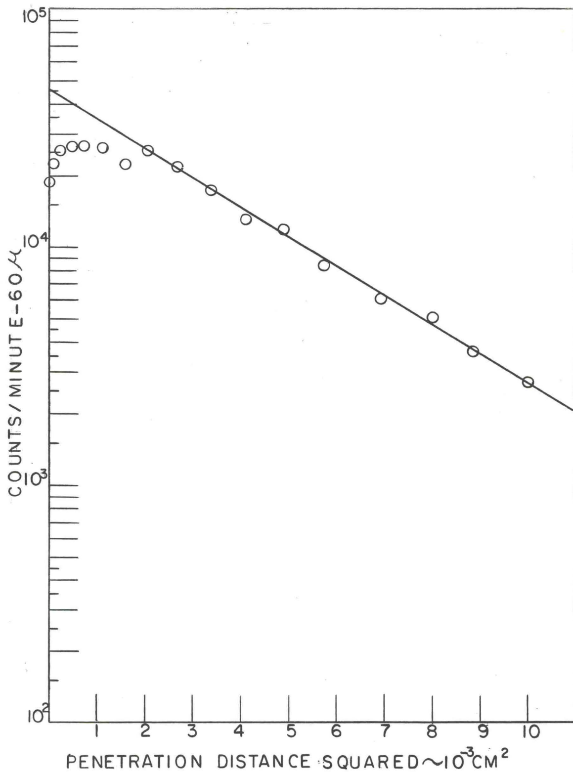
Figure 8. Solute Penetration Curve, Sample No. 88-- Annealed at 24 kb. pressure and 694°K for 1.63 \times 10^4 sec
